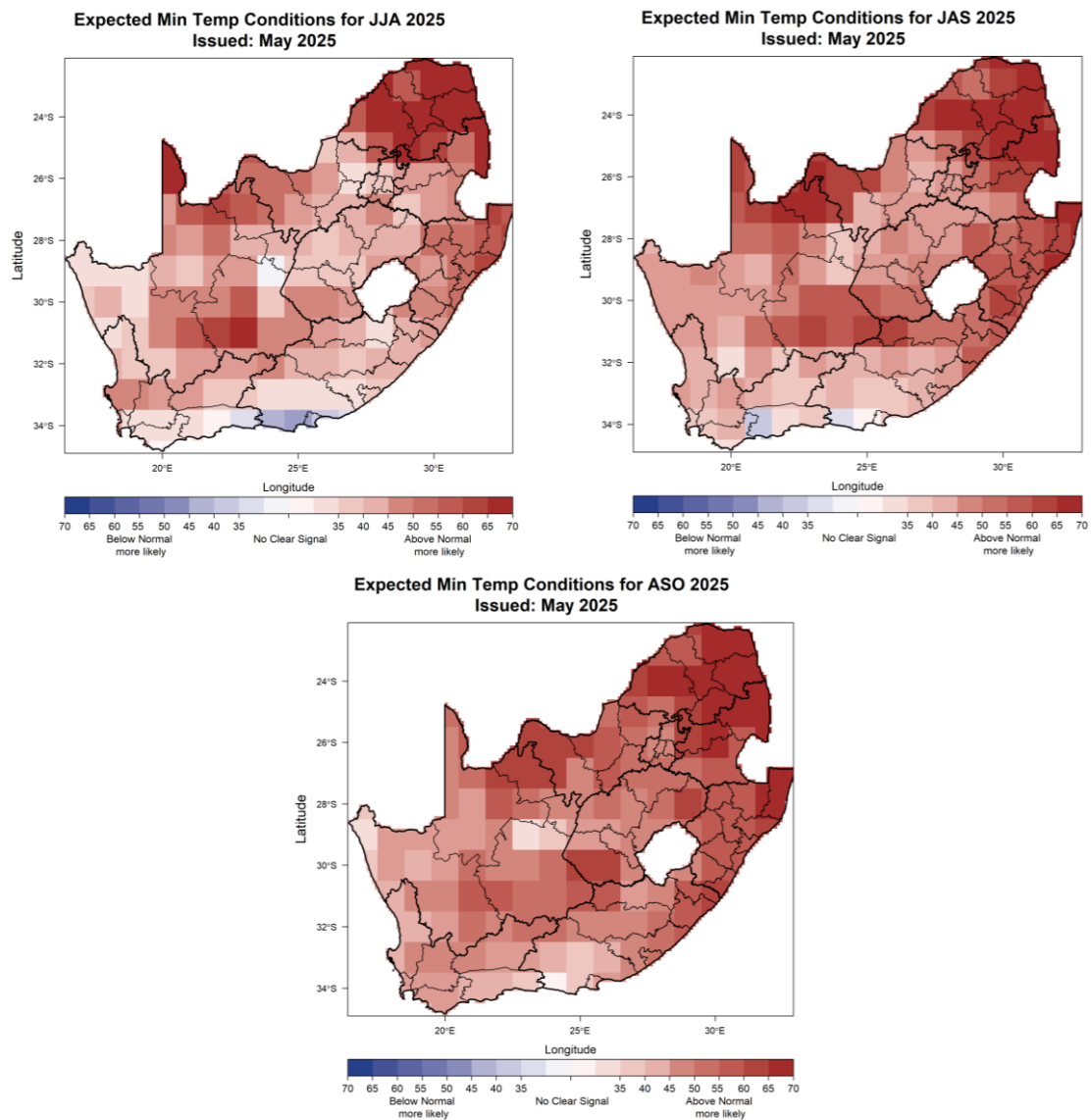
Figure 4: June-July-August 2025 (JJA; left), July-August-September 2025 (JAS; right), August-September-October 2025 (ASO; bottom) seasonal minimum temperature prediction. Maps indicate the highest probability of the above-normal and below-normal categories. Please refer to appendix Figure A2 for forecast skill levels.
