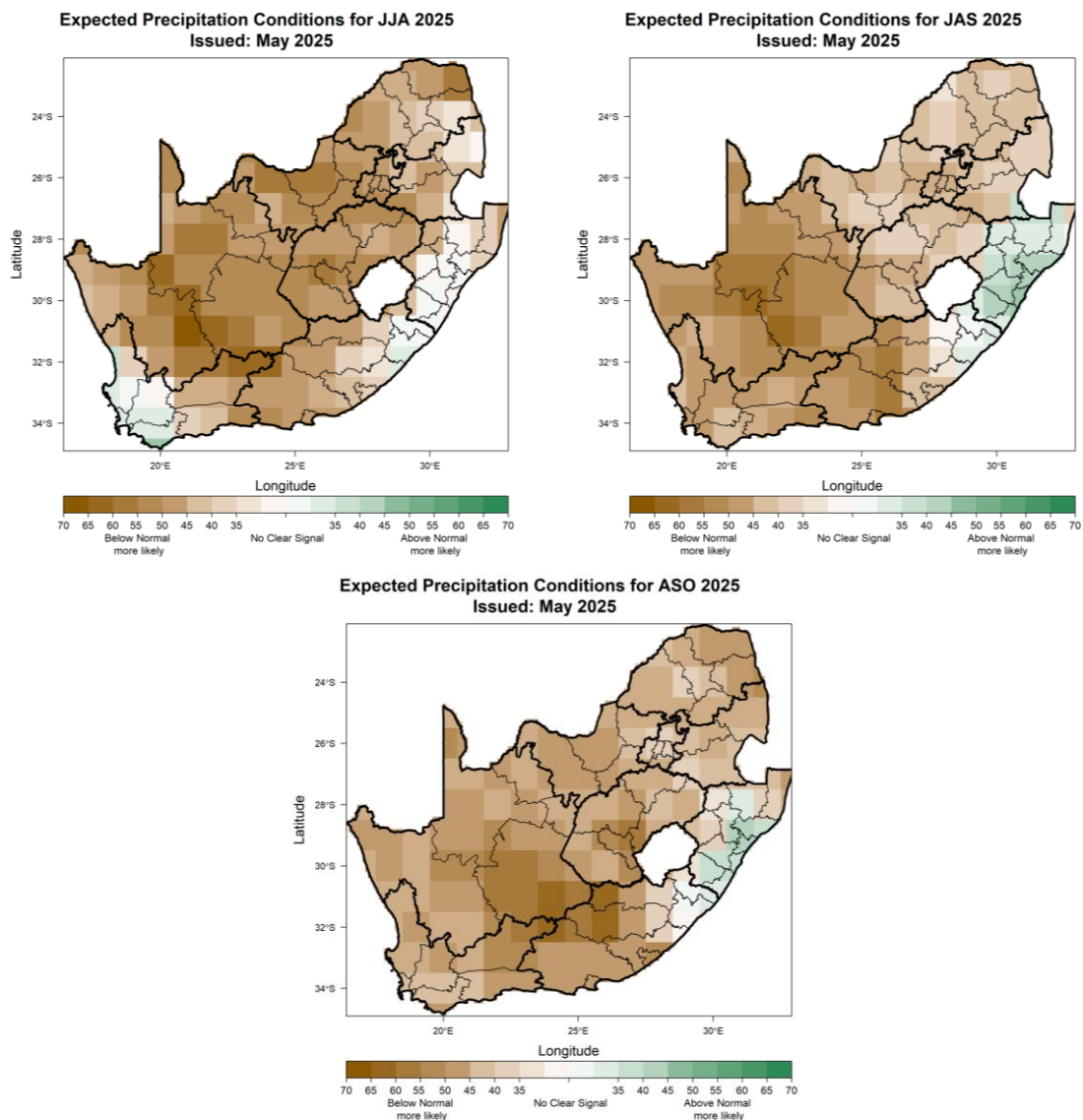
Figure 3: June-July-August 2025 (JJA; left), July-August-September 2025 (JAS; right), August-September-October 2025 (ASO; bottom) seasonal precipitation prediction. Maps indicate the highest probability of the above-normal and below-normal categories. Please refer to appendix Figure A1 for forecast skill levels.
