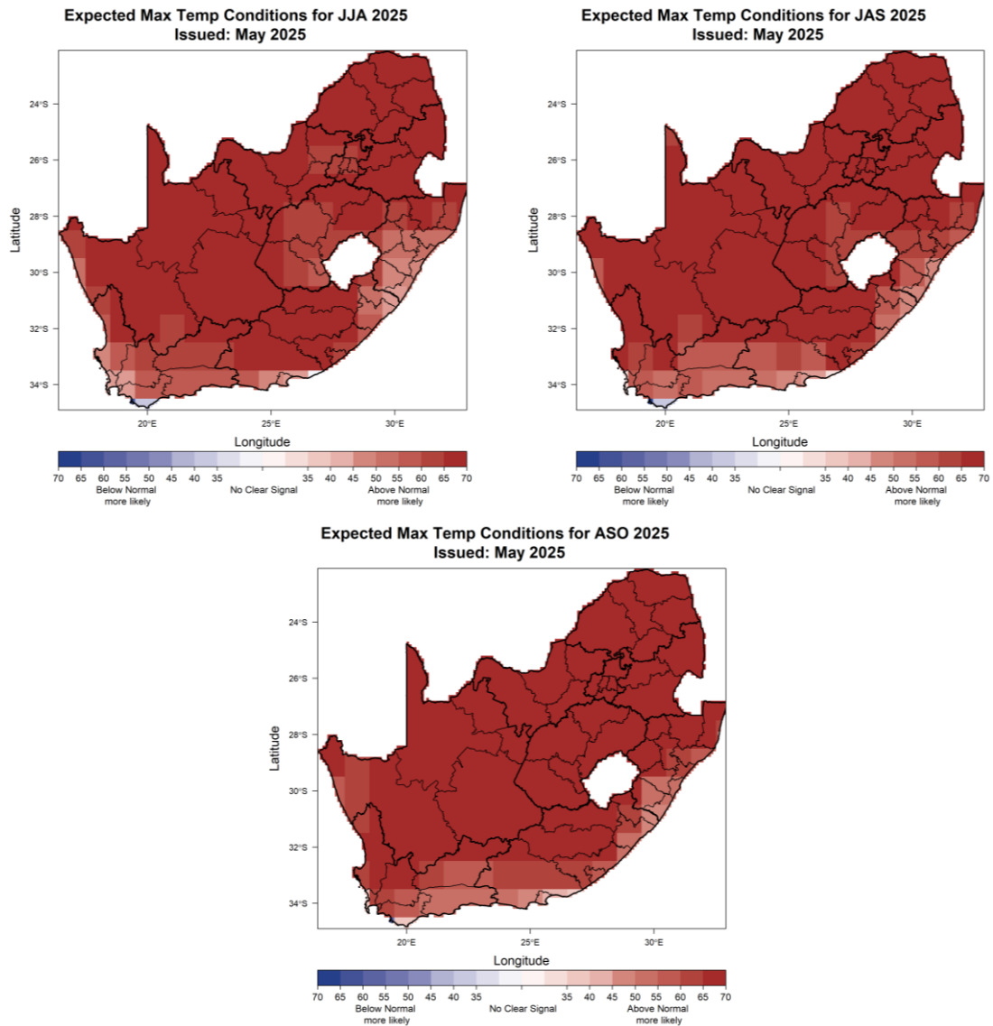
Figure 5: June-July-August 2025 (JJA; left), July-August-September 2025 (JAS; right), August-September-October 2025 (ASO; bottom) seasonal maximum temperature prediction. Maps indicate the highest probability of the above-normal and below-normal categories. Please refer to appendix Figure A3 for forecast skill levels.
