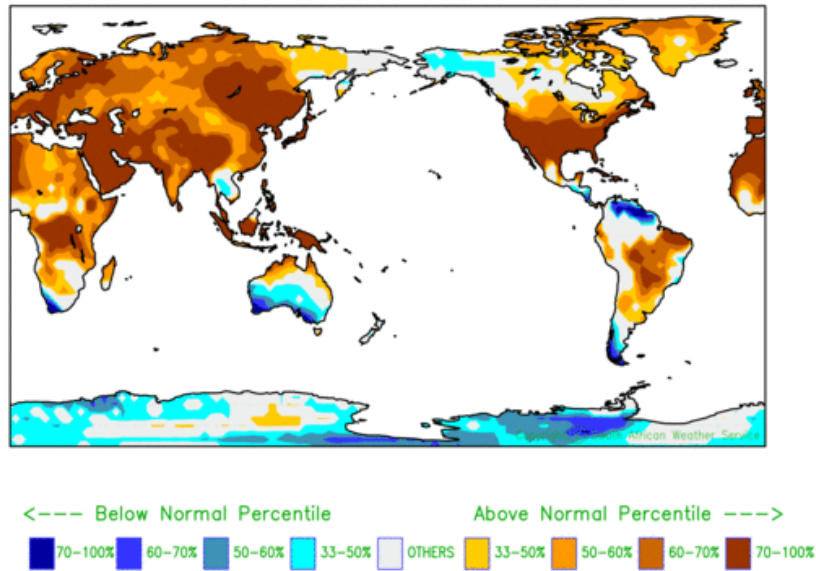
Figure 2: March-April-May, MAM (2025) global prediction for average temperature probabilities
