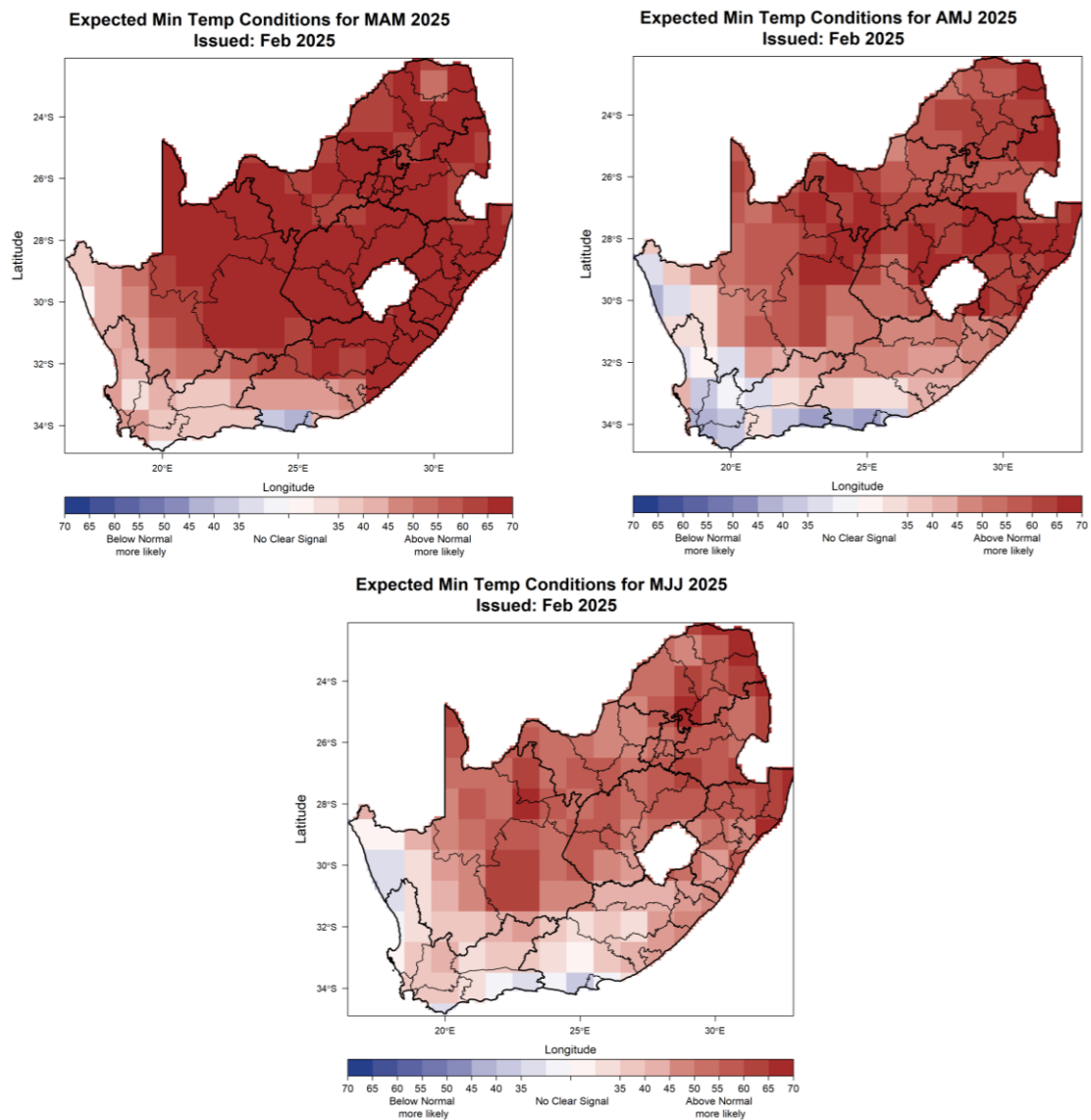
Figure 4: March-April-May 2025 (MAM; left), April-May-June 2025 (AMJ; right), May-June-July 2025 (MJJ; bottom) seasonal minimum temperature prediction. Maps indicate the highest probability of the above-normal and below-normal categories. Please refer to appendix Figure A2 for forecast skill levels.
