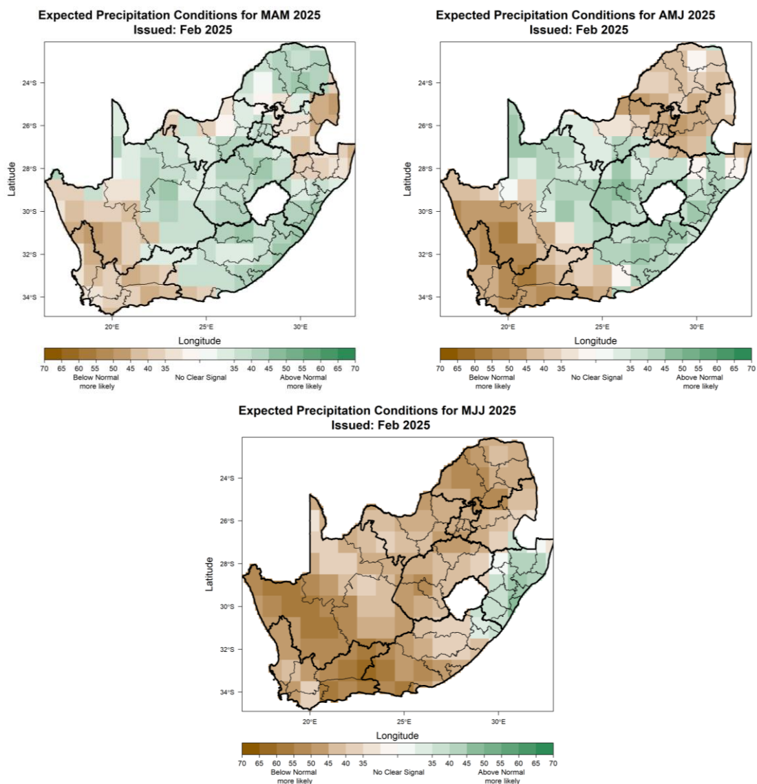
Figure 3: March-April-May 2025 (MAM; left), April-May-June 2025 (AMJ; right), May-June-July 2025 (MJJ; bottom) seasonal precipitation prediction. Maps indicate the highest probability of the above-normal and below-normal categories. Please refer to appendix Figure A1 for forecast skill levels.
