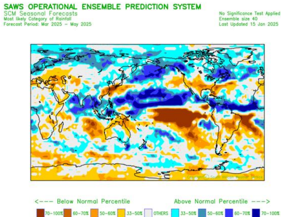
Figure 1: March-April-May, MAM (2025) global prediction for total rainfall probabilities
