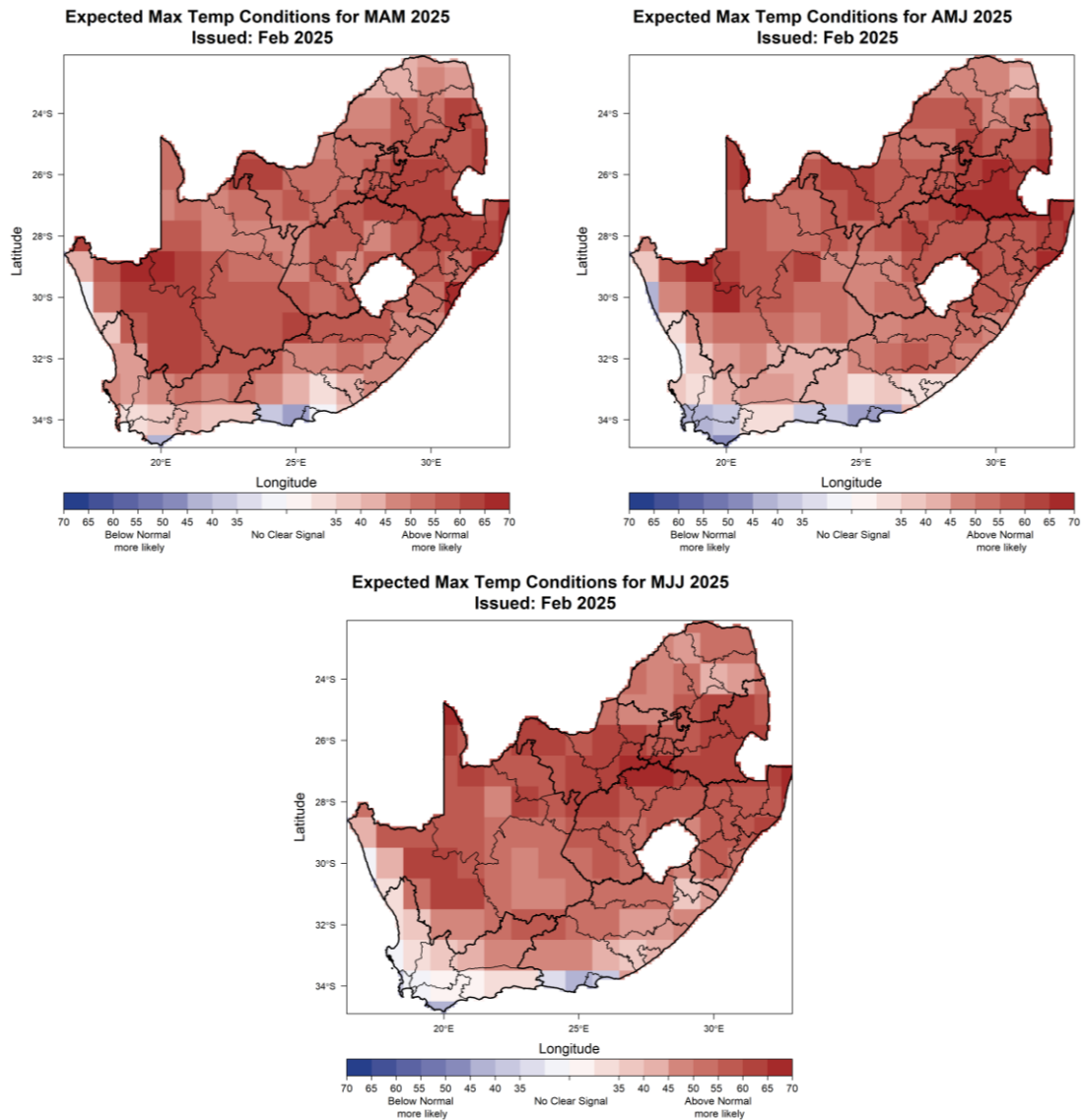
Figure 5: March-April-May 2025 (MAM; left), April-May-June 2025 (AMJ; right), May-June-July 2025 (MJJ; bottom) seasonal maximum temperature prediction. Maps indicate the highest probability of the above-normal and below-normal categories. Please refer to appendix Figure A3 for forecast skill levels.
