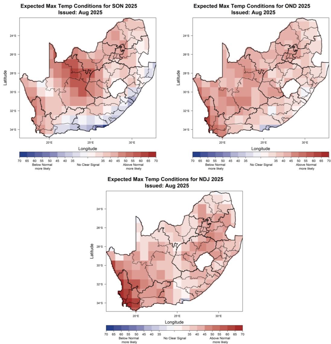
Figure 5: September-October-November 2025 (SON; left), October-November-December 2025 (OND; right), November-December-January 2025/26 (NDJ; bottom) seasonal maximum temperature prediction. Maps indicate the highest probability of the above-normal and below-normal categories. Please refer to appendix Figure A3 for forecast skill levels.
