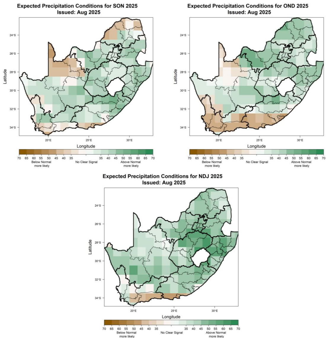
Figure 3: September-October-November 2025 (SON; left), October-November-December 2025 (OND; right), November-December-January 2025/26 (NDJ; bottom) seasonal precipitation prediction. Maps indicate the highest probability of the above-normal and below-normal categories. Please refer to appendix Figure A1 for forecast skill levels.
