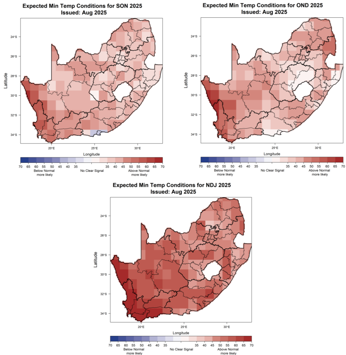
Figure 4: September-October-November 2025 (SON; left), October-November-December 2025 (OND; right), November-December-January 2025/26 (NDJ; bottom) seasonal minimum temperature prediction. Maps indicate the highest probability of the above-normal and below-normal categories. Please refer to appendix Figure A2 for forecast skill levels.
